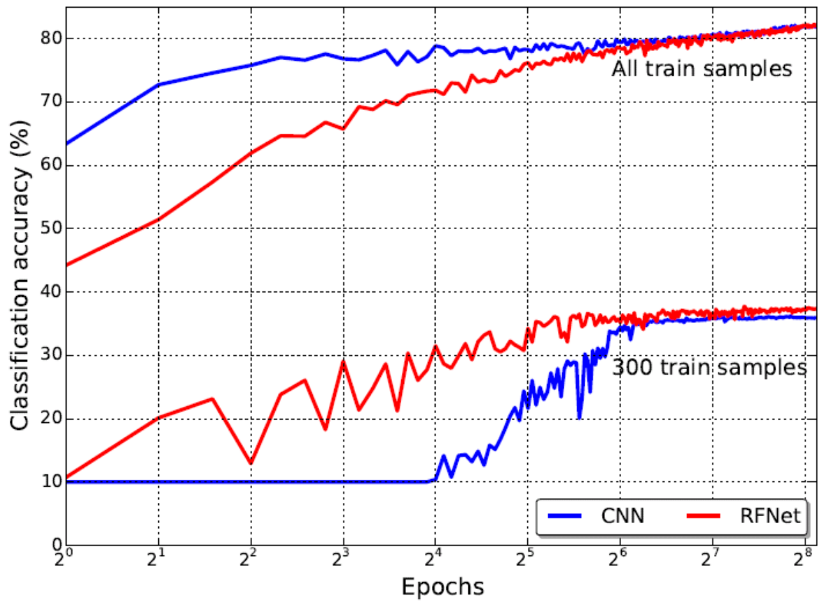
(a) CIFAR-10
